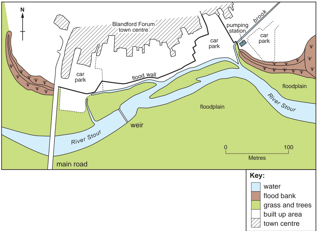
Fig. 1 The flood management scheme at Blandford Forum, Dorset
